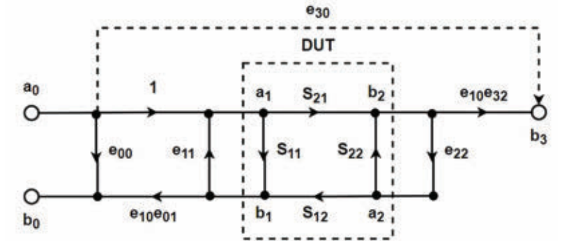
1. Our model starts with a perfect VNA. We create two error boxes and put them on either side of the DUT and attach the perfect VNA to the left and right sides. Images courtesy Copper Mountain Technologies
